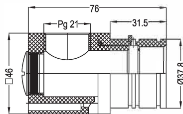
Female Housing
