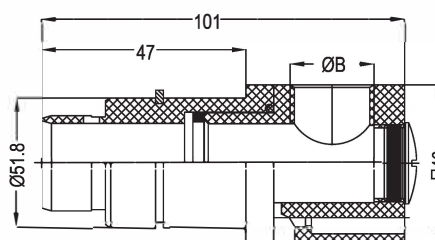
Male Housing
