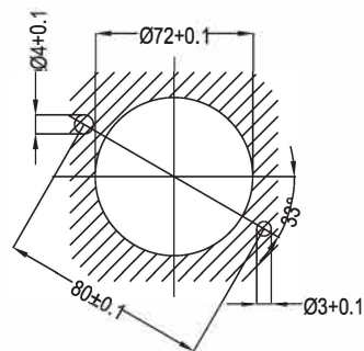
The front view of the mounting plate
