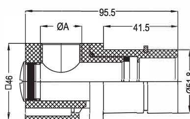
Female Housing
