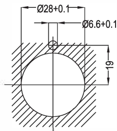
The front view of the mounting plate
