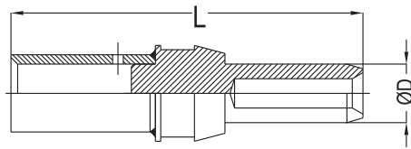
Pin Contact
