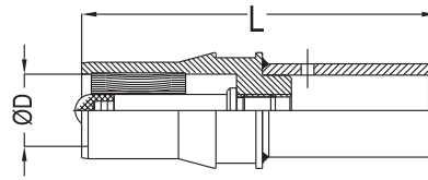
Socket Contact
