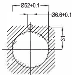
The front view of the mounting plate
