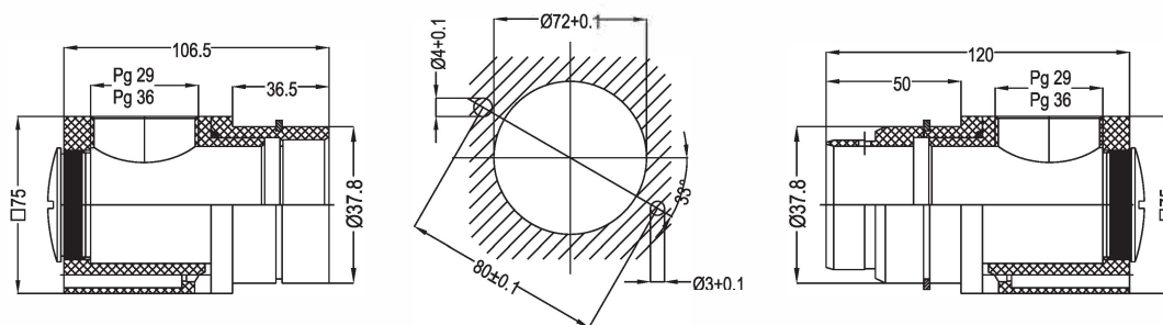
Female Housing
