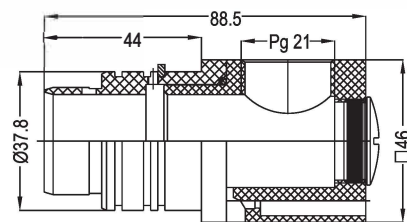
Male Housing
