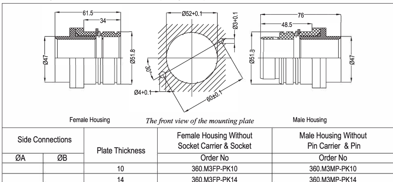
360-M3 Housing For Pin / Socket Carriers - 37mm ( Straight Port )
