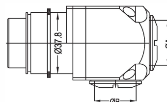
Male Housing
