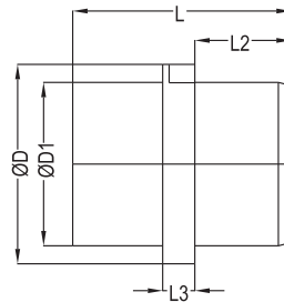
Socket Carriers (Socket Insulator)
