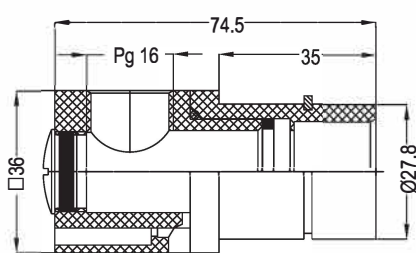
Female Housing
