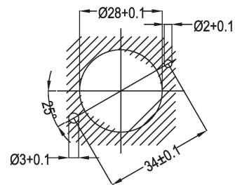
The front view of the mounting plate
