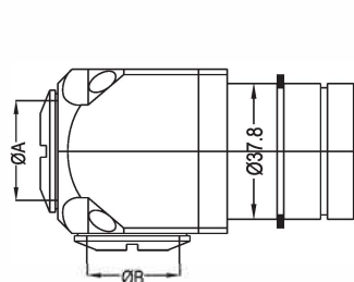
Female Housing
