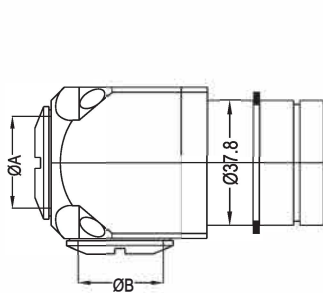
Female Housing
